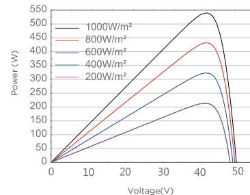
Current-Voltage Curve(MS565M-72H)
