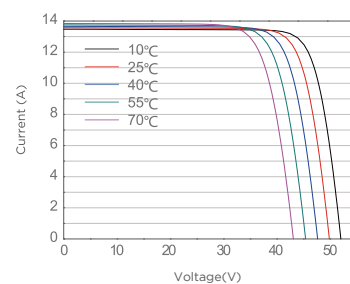
Current-Voltage Curve(MS565M-72H)
