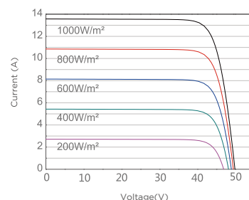
Current-Voltage Curve(MS565M-72H)
